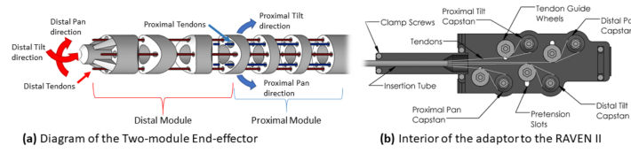
Figure 4: SnakeRaven macro-micro surgical manipulator concept razjigaev2021snakeraven.
